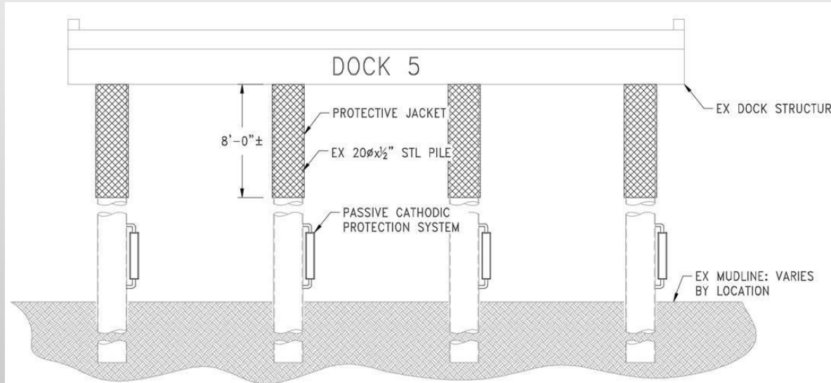
Dock 5 Corrosion Prevention Method
