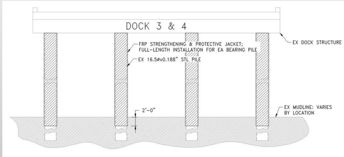
Docks 3 and 4 Pile Strengthening Methods
